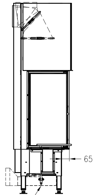
side view M~1:20
